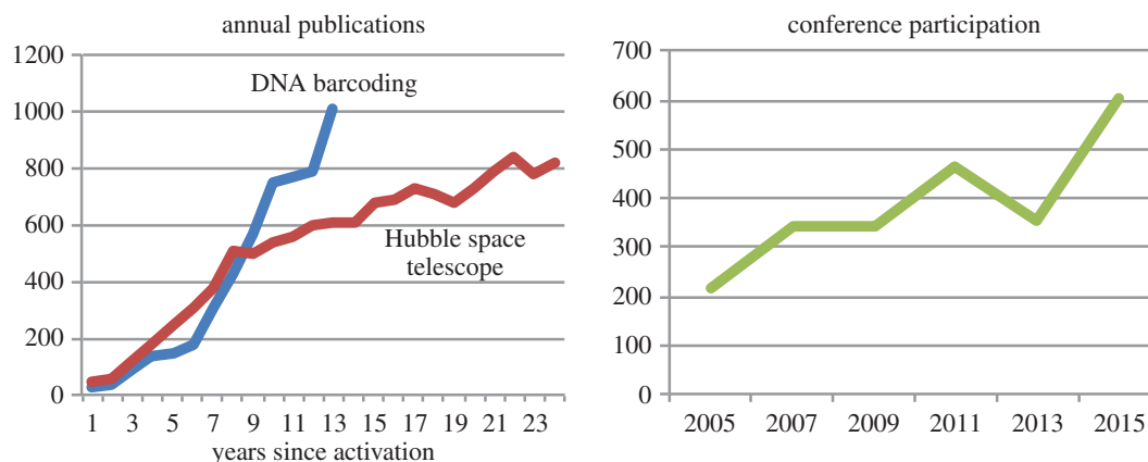
Figure 1. Metrics showing the growth of the DNA barcode research community through time as measured by the yearly number of publications on DNA barcoding and by the number of participants in the International Barcode of Life Conferences. Data on publication activity by the Hubble Space Telescope research community are presented for comparison.
