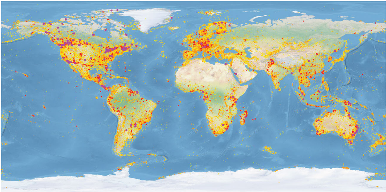
Figure 2. Heat map of the five million DNA barcode records in July 2016. Purple circles > 1000 records, red > 100 records, orange > 10 records, yellow 1–10 records.
